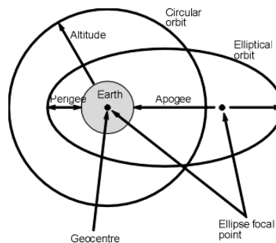
FIGURE 10 FIGURE CIRCULAR AND ELLIPTICAL ORBITS SHAPES
