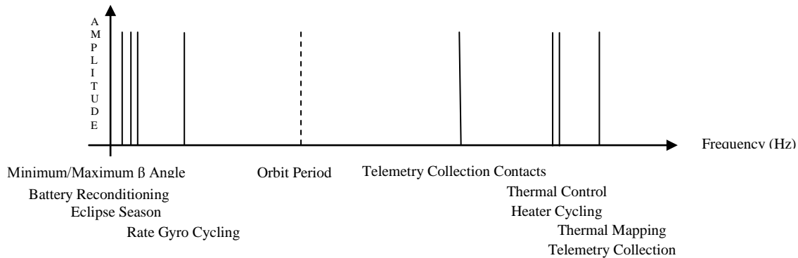
FIGURE 11 FREQUENCY SPECTRUM (POSITIVE FREQUENCIES) FOR BOEING GPS BLOCK I SATELLITE IN MEDIUM EARTH ORBIT
