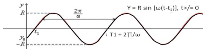
FIGURE 3 HARMONIC FUNCTION
