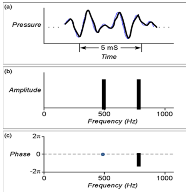
FIGURE 5 ANALOG ELECTRONIC MEASUREMENT SINUSOIDAL BEHAVIOR AND ITS FREQUENCY AND PHASE SPECTRUM
