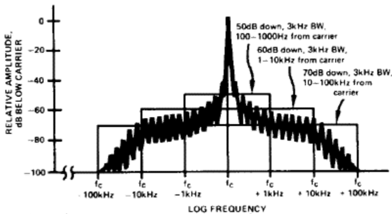
FIGURE 2 POWER SPECTRAL DENSITY (PSD) FOR AN RF SIGNAL
