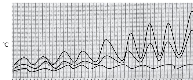
FIGURE 10 MINIMUM, AVERAGE AND MAXIMUM TELEMETRY VALUES FOR THE 4 YEAR LIFE OF GPS SATELLITE IN 12 HOUR ORBIT WITH 2 ORBITS PER DAY WITHOUT EQUIPMENT CYCLING
