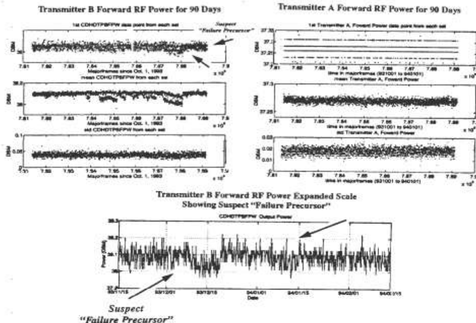
Figure 1. EUVE Transmitter A and B Forward RF Power FPP Plots
