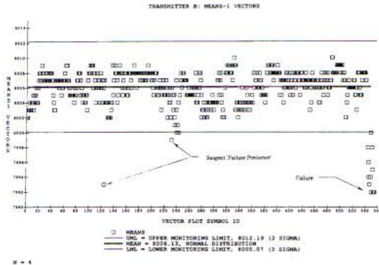
Figure 5. Statistical Pattern Recognition Vectors for EUVE Transmitter B
