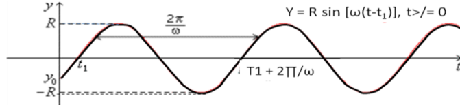
FIGURE 3 HARMONIC FUNCTION
